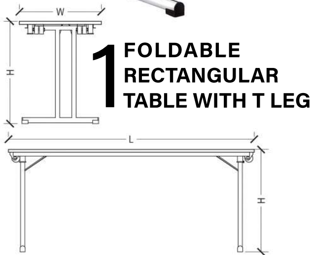
DIMENSIONS (MM) RECTANGULAR TABLE
